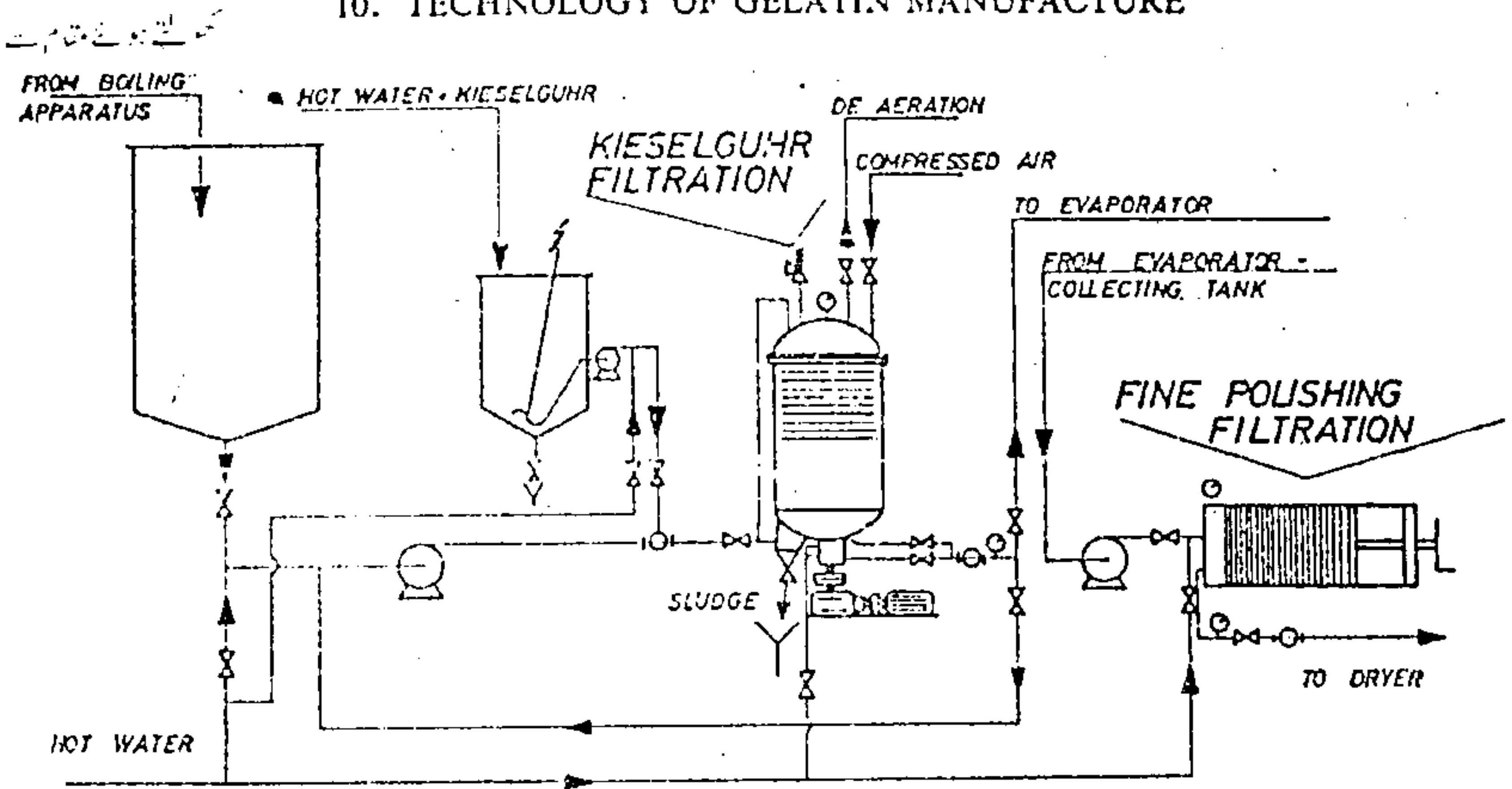
FIG. Flow diagram—gelatin filtration system "Sohenk-Fitterbau."
