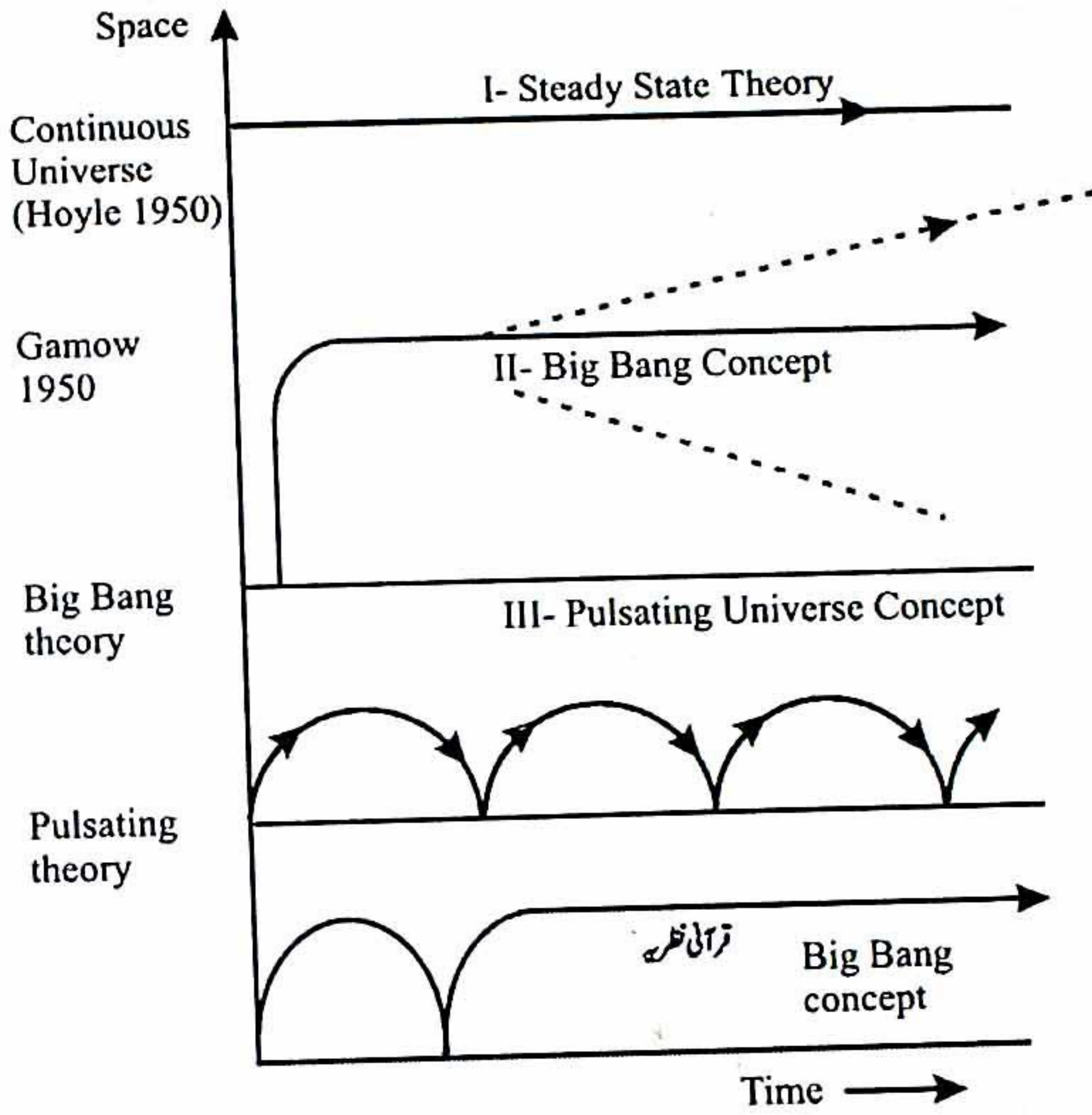
Fig. 1: Concepts of the Creation of Universe
